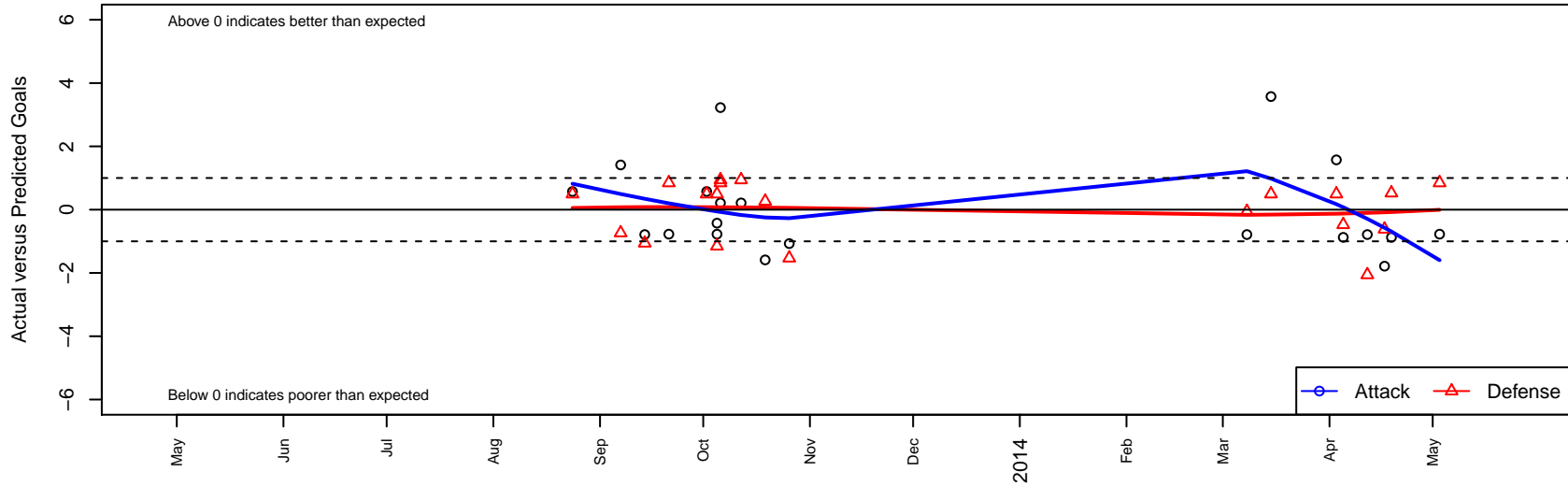
Indie Chicas G02 Dots are actual minus expected GF (blue circles) and GA (red triangles). Blue line is smoothed change in attack strength. Red is smoothed change in defense strength.
